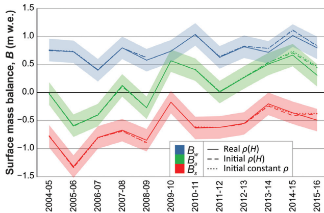
Fig. 8. Winter ( B_w ), summer ( B_s ) and annual ( B_a ) SMBs for all three density scenarios used in Table 2. The shadings indicate the error bars for the SMB values calculated using the real density vs. depth function \rho(H) . Modelled values for 2009–10 have been excluded consistently with Table 2.
