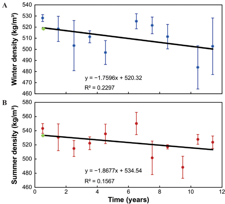
Fig. 3. Temporal evolution of the end-of-winter averaged (A) and end-of-summer averaged (B) snow density for the period 2004–2016 (time given in years counted from the start of the hydrological year 2005, i.e. 1 April 2004), with their linear trends illustrated by the corresponding least-square fits. The error bar for each data point is the standard error of the mean density of the year. The density data point for the hydrological year 2010 has been excluded as outlier, because the individual values making up the average for this year are inconsistent, suggesting experimental errors during fieldwork. The data point for the winter of the hydrological year 2014 is unavailable because in that year there was a single set of density measurements, at the end of the summer season. The green diamonds correspond to \hat{\rho}_w^{\text{init}} and \hat{\rho}_s^{\text{init}} .
