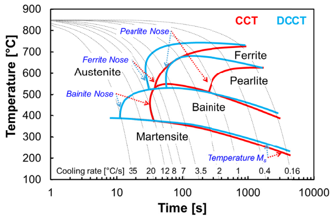
Fig. 2. Comparison of CCT and DCCT transformation diagrams of steel 20MnCrS5
