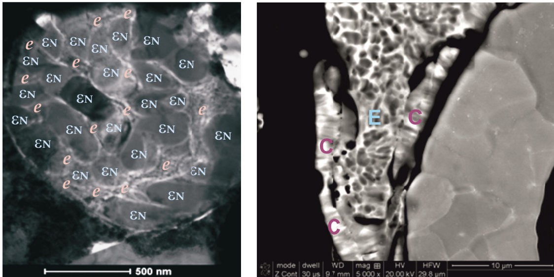
Fig. 4. Morphology of the Fe-Al coating deposited on the steel substrate by the D-Gun method, (coating about 100 μm thick formed from the Fe-Al powder containing particles of 40-75 μm in diameter), a/ cells of the \epsilon_N -phase surrounded by the eutectic precipitates, b/ E – an eutectic formed during rapid solidification; C – columnar morphology localized in the vicinity of the eutectic precipitates and growing in two different directions
