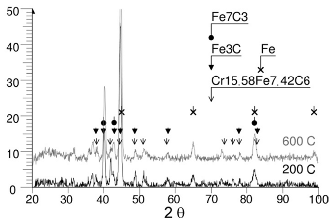
Fig. 7. XRD patterns for investigated cast steel after tempering (i.e.: 200, 600°C)
