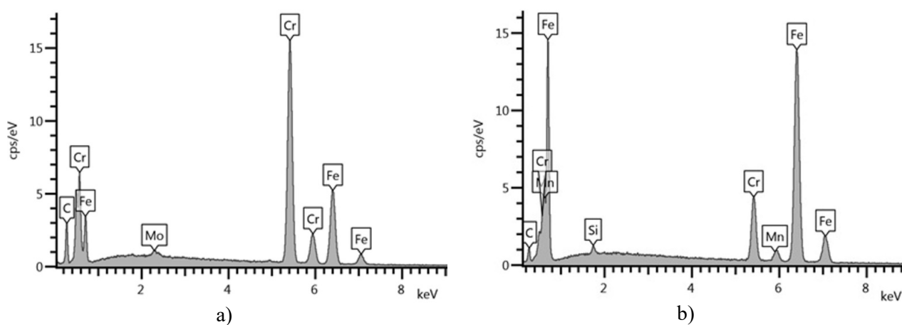
Fig. 3. X-ray diffraction pattern and EDS spectra showing the area of eutectic precipitates in Fig. 2a, area 1 – a) and cast steel matrix in Fig. 2a, area 2 – b)
