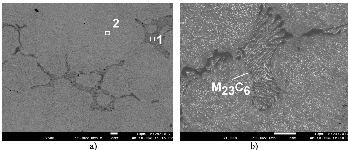
Fig. 2. Microstructure of investigated cast steel – sample H2, discontinuous eutectic carbides network, a) magn. 500 \times , b) magn. 1500 \times
