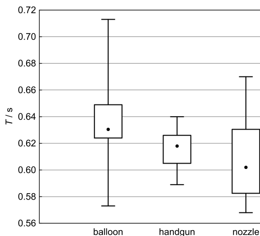
Fig. 9. Quartiles of the reverberation times for the 1/3 octave band with 2 kHz center frequency, determined in the stockroom. Sound generated by the three compared sources: points – medians, boxes – 25% to 75% range, whiskers – full range.
