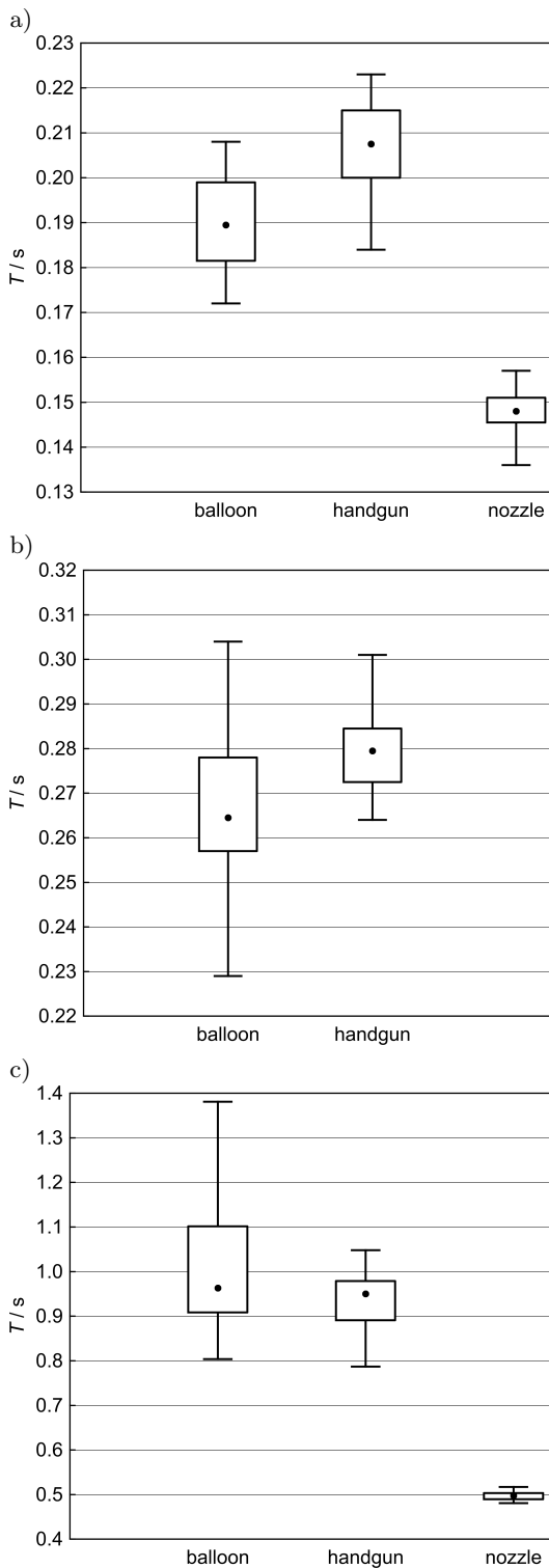
Fig. 6. Quartiles of the reverberation times assessed with the three compared sound sources in three rooms: a) small room, b) medium-sized room, c) stockroom. Points – medians, boxes – 25% to 75% range, whiskers – full range.
