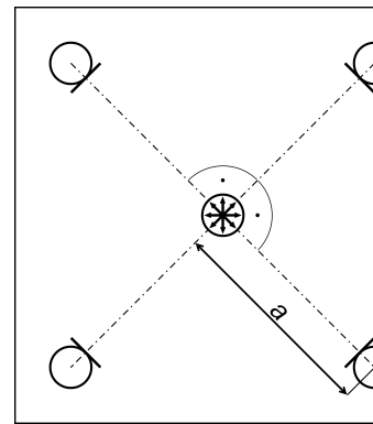
Fig. 1. Experimental setup: four microphones around the acoustic signal source; a \approx 2 m except the small room where a \approx 1 m. Distances to the room walls are not in the picture scale.
