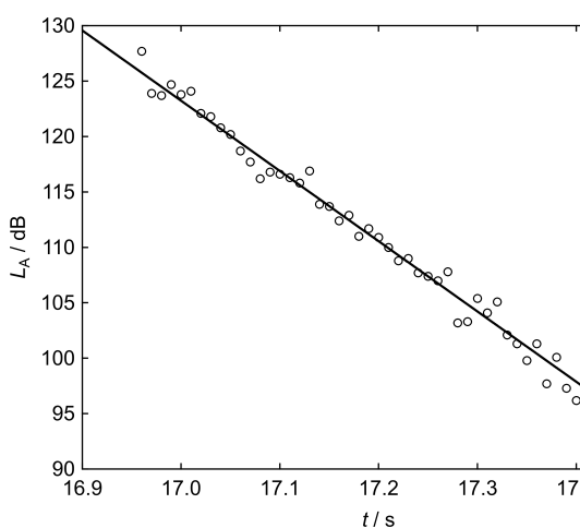
Fig. 5. Linear decrease of the sound level after firing the handgun; points – experimental values; line – simple linear regression (Eq. (1)).
