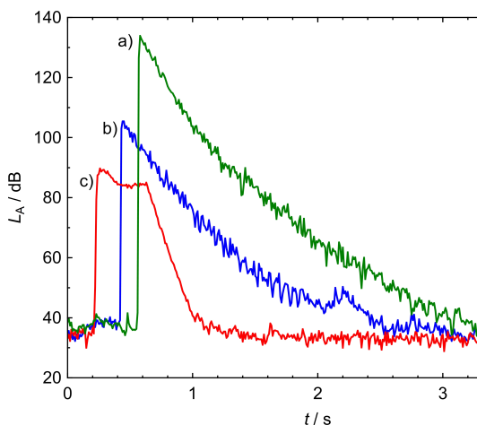
Fig. 4. Sound level vs. time curves obtained using three sound sources in the stockroom: a) a gunshot, b) a balloon burst, c) a compressor nozzle hiss.
