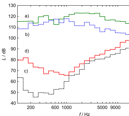
Fig. 2. Frequency characteristics of the sources in 1/3 octave bands: a) a gunshot, b) a balloon burst, c) a compressor nozzle hiss recorded in the stockroom, d) a hiss recorded in the small room using measuring set #2.
