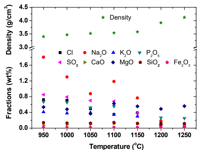
Fig. 5. True densities ( \text{g/cm}^3 ) and impurities fractions (wt%) in form of stable oxides, except for Cl, of alumina from calcinated ACH in a step of 50°C from 950 to 1250°C
