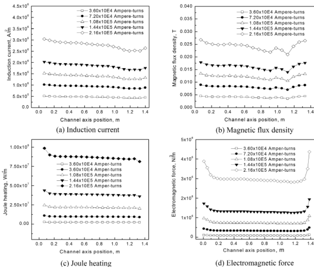
Fig. 9. Magnetic variable at line of y = 0.05 m under different condition of Power
