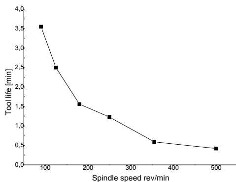
(c) Effect of spindle speed on life of tool at constant feed rate of 0.32 \text{ mm/rev}
