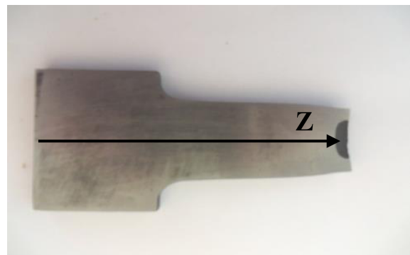
Fig. 4. Plastically deformed specimen.
