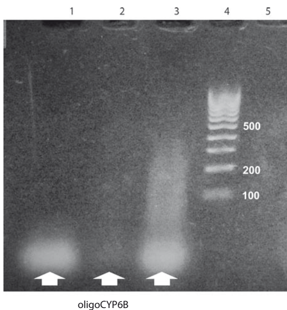
Fig. 1. Electrophoregram (1.8% agarose gel) representing activity of intracellular nucleases of Leptinotarsa decemlineata and L. dispar for 60 min at 27°C: 1 – control (10 µl oligoCYP6B at a concentration of 100 pmol · µl -1 ); 2 – tissue homogenate of L. decemlineata (1.5 mg of biomass per 10 µl of TE buffer, pH 7.4) + 10 µl oligoCYP6B at a concentration of 100 pmol · µl -1 ; 3 – tissue homogenate of L. dispar (1.5 mg of biomass per 10 µl of TE buffer, pH 7.4) + 10 µl oligoCYP6B at a concentration of 100 pmol · µl -1 ; 4 – DNA ladder (100 kb); 5 – tissue homogenates of L. decemlineata (1.5 mg of biomass per 10 µl of TE buffer, pH 7.4) and L. dispar (1.5 mg of biomass per 10 µl of TE buffer, pH 7.4) without treatments
