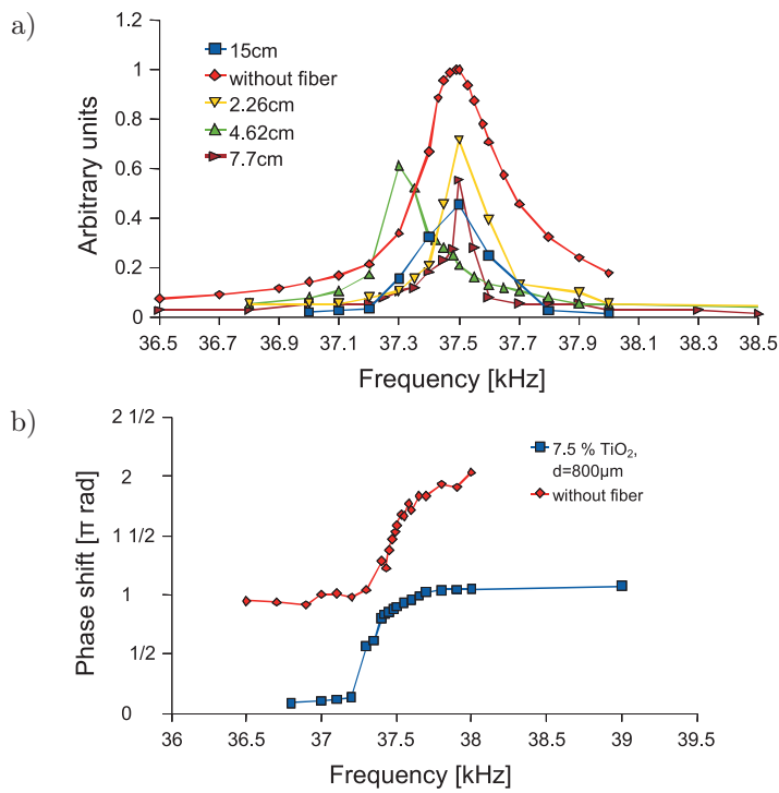
Fig. 2. Relation of output signal amplitude depending on frequency and optical fibre length (a) and phase shift between input and output signal for a 7.7 cm long fibre doped with TiO 2 (b), without fiber – when fiber is not glued to the transducer, output signal amplitude was measured at the end of the transducer.
