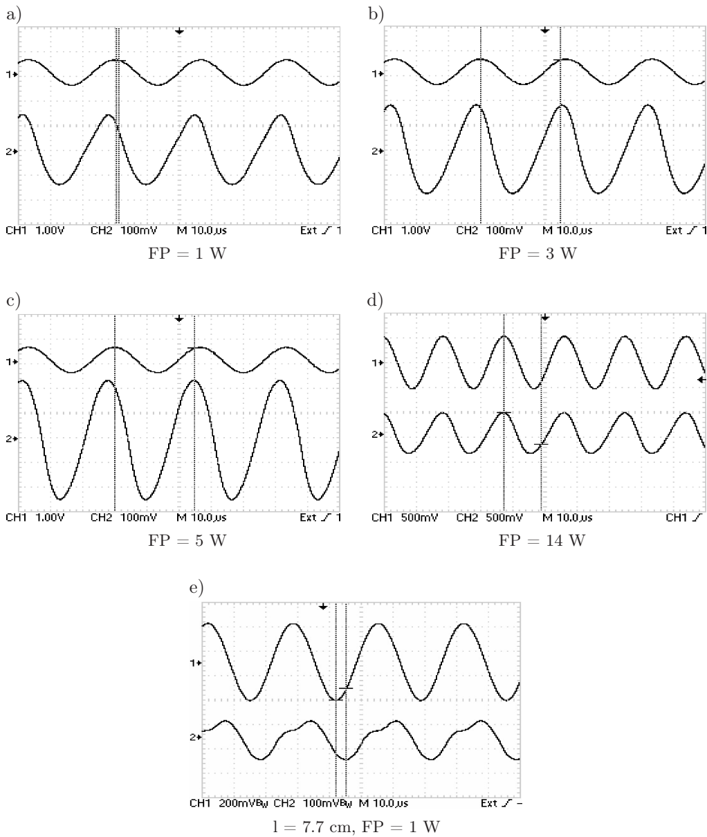
Fig. 5. Relation of the shape of output signal to the length of the optical fibre and transducer forward power FP: a), b), c), d) for an optical fibre doped by 7.5% of TiO 2 , the length of which is l = 15 cm, e) for an optical fibre with 3% of GeO 2 , CH1 – input signal, CH2 – output signal.
