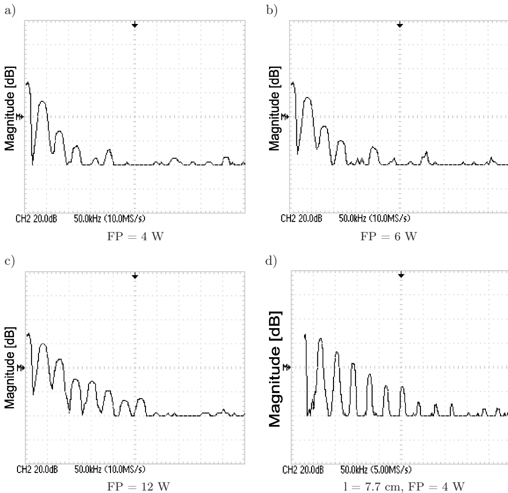
Fig. 7. The dependence of the output signal spectrum on the power applied to the transducer, a) FP = 4\text{ W} , for an optical fibre length l = 4.6\text{ cm} doped by 7.5% of TiO_2 , b) FP = 6\text{ W} , for an optical fibre length l = 4.6\text{ cm} doped by 7.5% of TiO_2 , c) FP = 12\text{ W} , for an optical fibre length l = 4.6\text{ cm} doped by 7.5% of TiO_2 , d) FP = 4\text{ W} for an optical fibre length l = 7.7\text{ cm} doped by 3% of GeO_2 .
