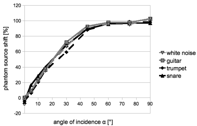
Fig. 13. Localization curves for ORTF for 60° basis separately for all sound sources.
