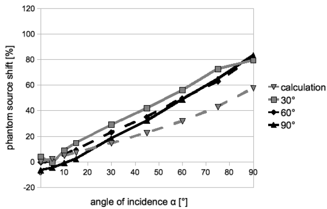
Fig. 7. Localization curves for XY (90°) for different bases averaged for all sound sources compared with calculated results.
