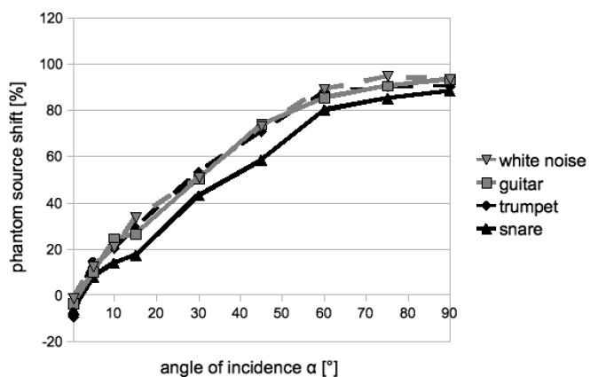
Fig. 11. Localization curves for AB (20 cm) for 60° basis separately for all sound sources.
