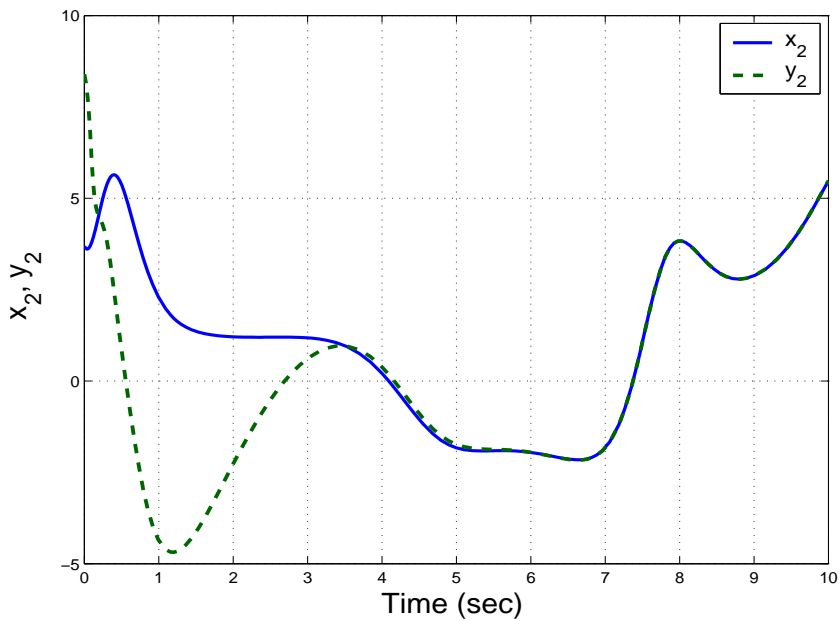
Figure 7: Synchronization of the states x_2(t) and y_2(t)
