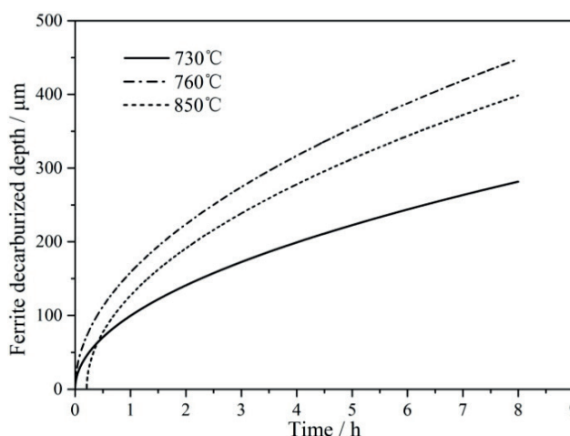
Fig. 13. The ferrite decarburization depth - soaking time curves at 730 °C, 760 °C and 850 °C
