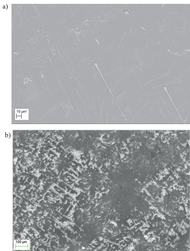
Fig. 3. Surface view of AC-AlSi12 alloy before (a) and after oxidizing (b)
