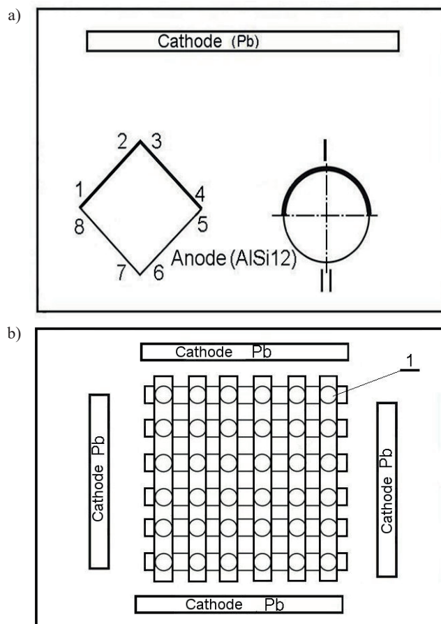
Fig. 1. Influence of skeleton's element position versus cathode on the structure of oxide coating: a) using one cathode, square and cylindrical connector rod; b) using four cathodes, 1 – cast skeleton being oxidized.
