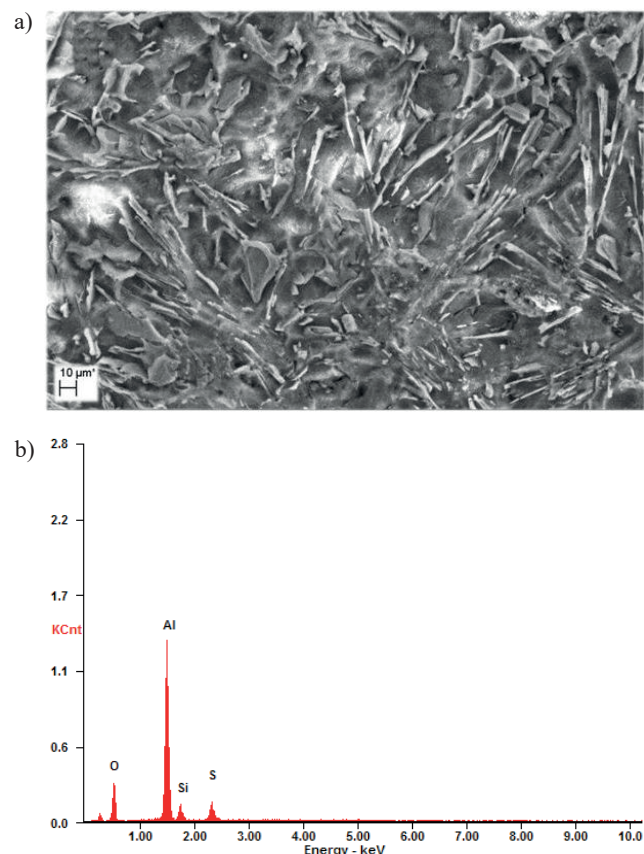
Fig. 4. Surface view of AC-AlSi12 alloy after oxidizing (a) and quantities of chosen elements at point 1 (b)
