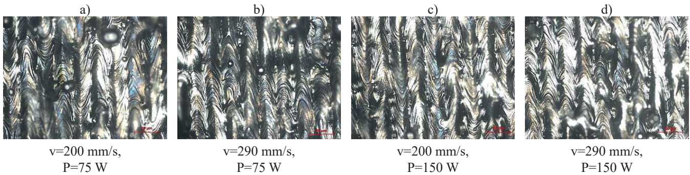
Fig. 4. Light microscope images represent the differences of SLM parts made with different values of laser power and scanning speed, mag. 1000x
