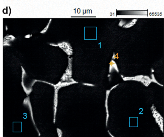
Fig. 2. Typical microstructure of investigated billets in as-cast state
