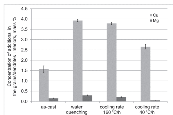
Fig. 4. Concentration of Cu and Mg in the dendrites/grains interiors in as-cast state and after homogenization (mean values from ten measurements in randomly selected areas)
