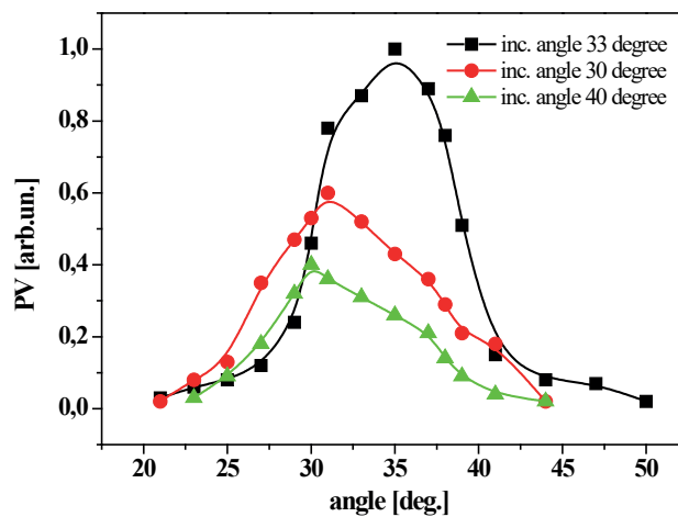
Fig. 7. Angular dependence of PV efficiency for CZTS nanocomposites
