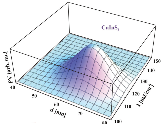
Fig. 6. Laser induced dependence for the PV efficiency for the \text{CuInS}_2 nanofilms
