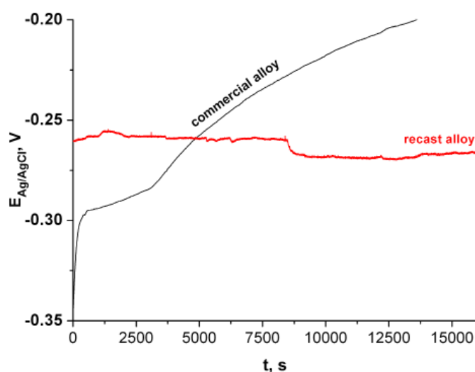
Fig. 3. Evolution of open circuit potential of tested alloy
