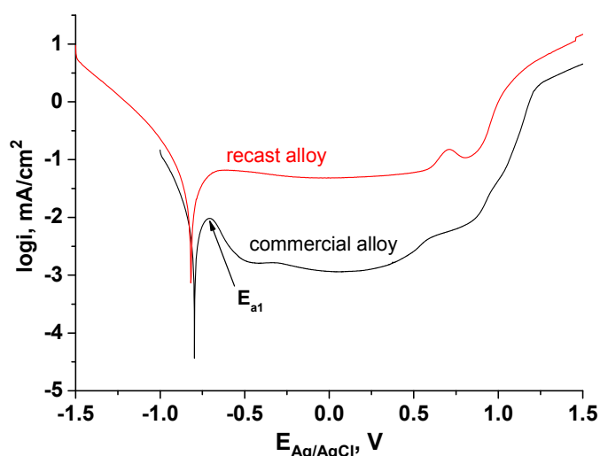
Fig. 4. Polarization curves of tested samples
