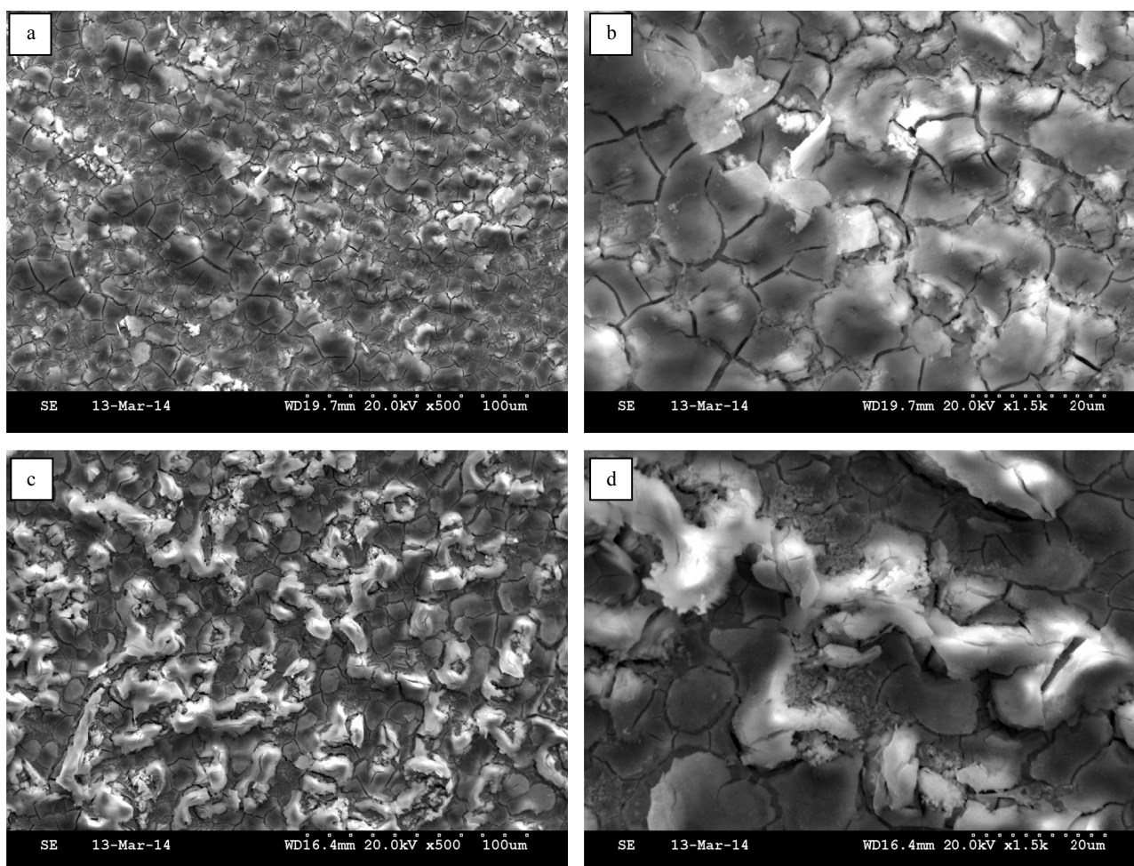
Fig. 5. SEM images of Ni-Cr-Mo alloy after polarization test; alloy; a=b commercial alloy, c=d recast alloy
