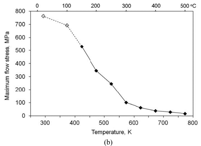
Fig. 2. Effect of deformation temperature on the flow stress characteristics observed for as extruded Ag/Al alloy: (a) \sigma_t - \varepsilon_t curves observed at deformation temperature marked in the figure; (b) effect of deformation temperature on the flow stress maximum detected during compression test
