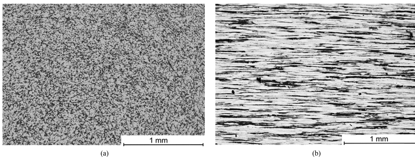
Fig. 5. SEM microstructure of as-extruded Ag/Al composite: a) cross-sectioned rod; b) longitudinally sectioned rod
