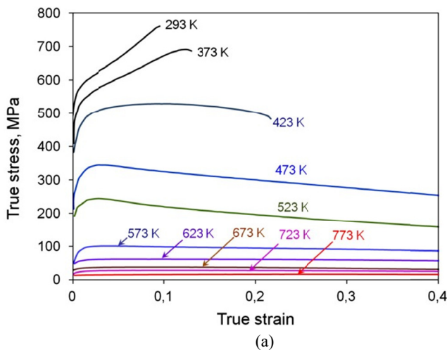
Fig. 2. Effect of deformation temperature on the flow stress characteristics observed for as extruded Ag/Al alloy: (a) \sigma_t - \varepsilon_t curves observed at deformation temperature marked in the figure; (b) effect of deformation temperature on the flow stress maximum detected during compression test
