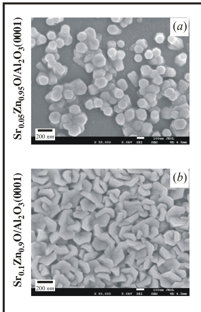
Fig. 6. Scanning electron microscopy images of a) \text{Sr}_{0.05}\text{Zn}_{0.95}\text{O}/\text{Al}_2\text{O}_3(0001) ; and b) \text{Sr}_{0.1}\text{Zn}_{0.9}\text{O}/\text{Al}_2\text{O}_3(0001) . Both films were grown at T = 650^\circ\text{C} under 0.5 Torr \text{O}_2 background pressure
