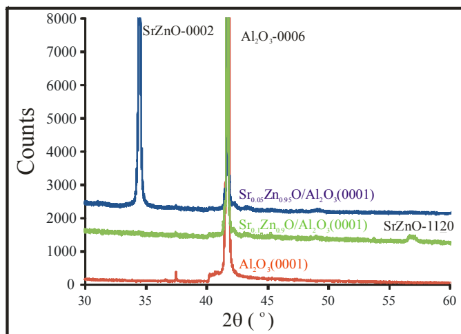
Fig. 7. XRD spectra of \text{Al}_2\text{O}_3(0001) and \text{Sr}_{0.05}\text{Zn}_{0.95}\text{O} , and \text{Sr}_{0.1}\text{Zn}_{0.9}\text{O} grown on \text{Al}_2\text{O}_3(0001) at T = 750^\circ\text{C} under 0.5 Torr \text{O}_2 background pressure
