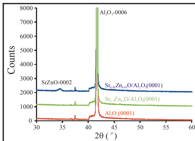
Fig. 1. XRD spectra of Al 2 O 3 (0001) and Sr 0.05 Zn 0.95 O and Sr 0.1 Zn 0.90 O grown on Al 2 O 3 (0001) at T = 380°C under 15 mTorr O 2 background pressure
