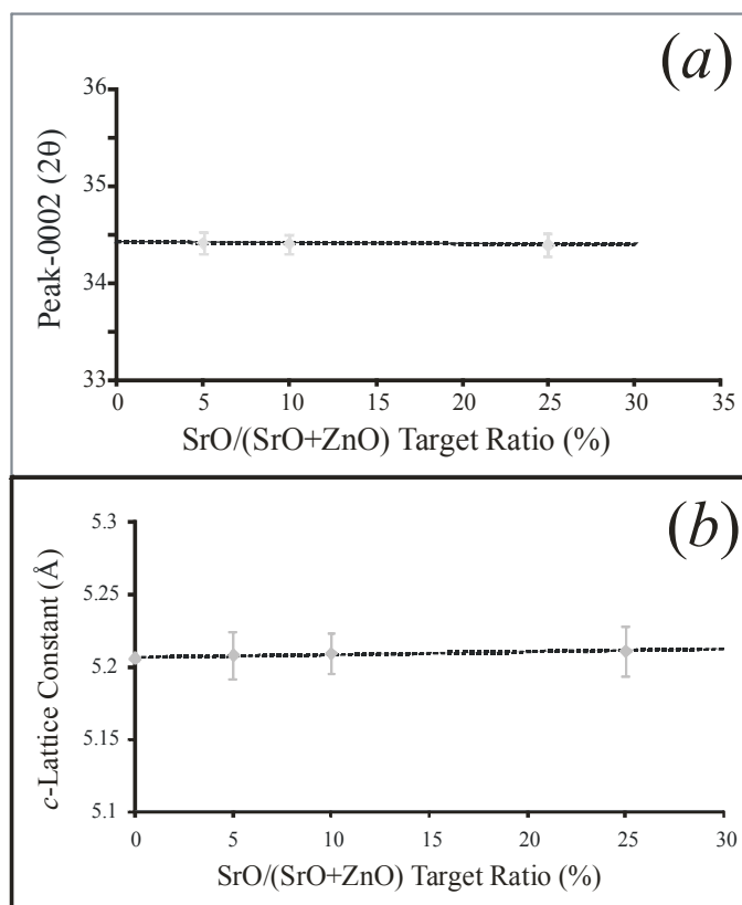
Fig. 4. Peak positions and c -lattice constants of SrZnO alloy as a function of SrO ratio ( x )
