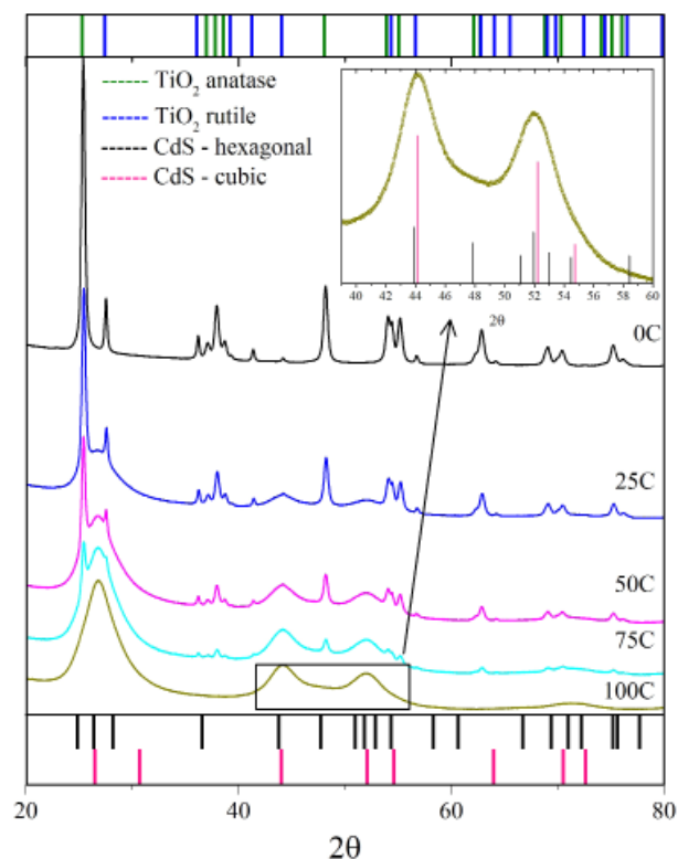
Fig. 4. X-ray diffraction patterns of TiO 2 /CdS nanopowders. Inset: 2θ range between 39-60°
