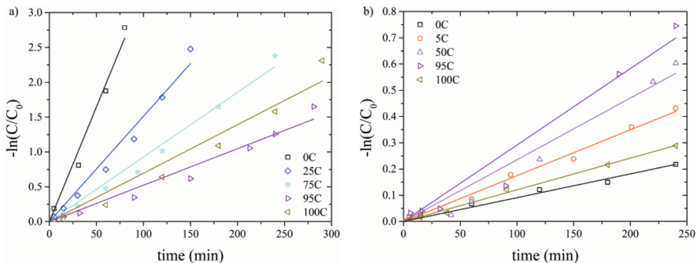
Fig. 8. First-order kinetics of methyl orange degradation using TiO 2 and CdS nanoparticles and TiO 2 /CdS nanocomposites as the catalyst under UV (a) and UV-vis (b) irradiation
