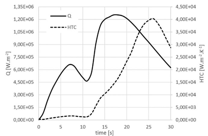
Fig. 9. Heat flux and HTC at pouring temperature 670°C and pressure 150 MPa
