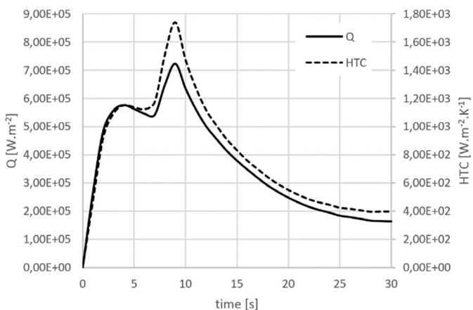
Fig. 6. Heat flux and HTC in gravity casting at pouring temperature 710°C
