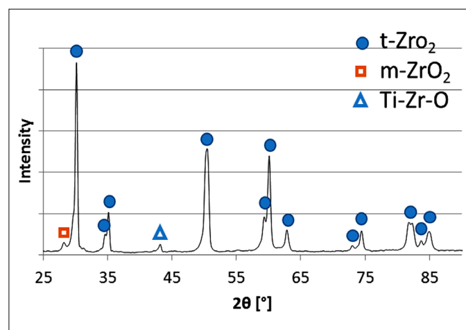
Fig. 2. X-Ray diffraction spectra of the cross section of ZrO_2 + 10 \text{ vol.}\% \text{ Ti} composite
