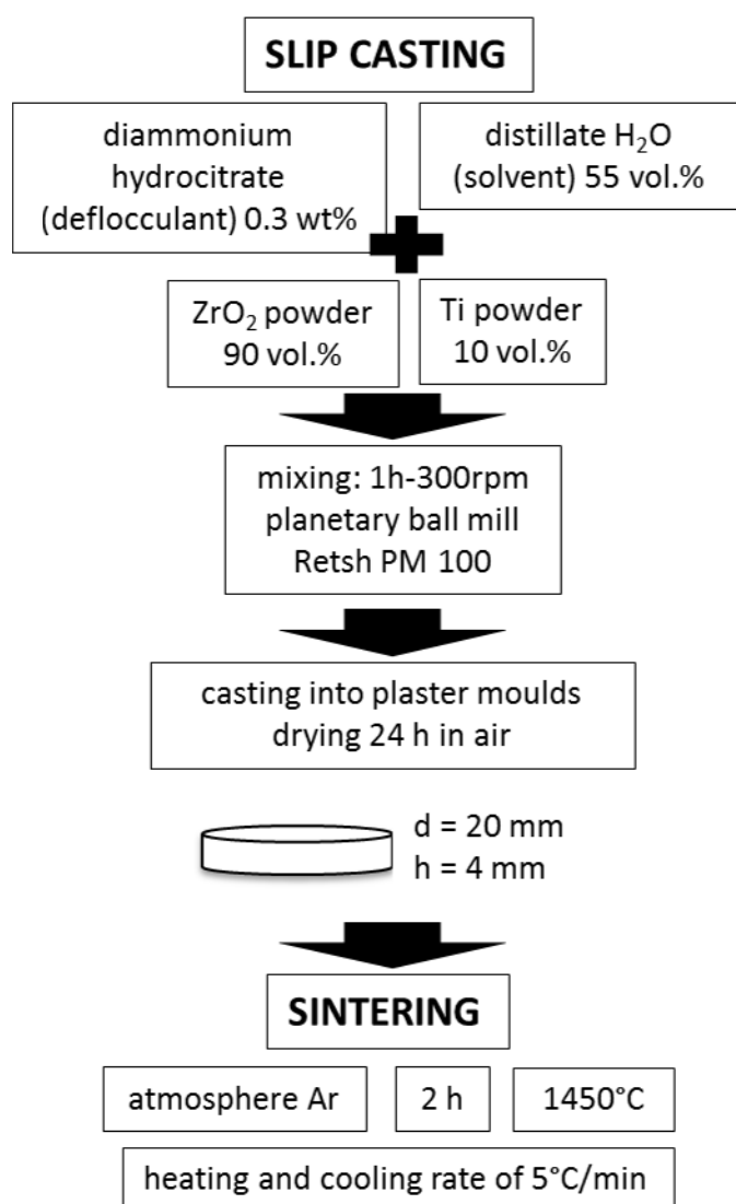
Fig. 1. Scheme of the ZrO_2 - 10 \text{ vol.}\% \text{ Ti} composite formation
