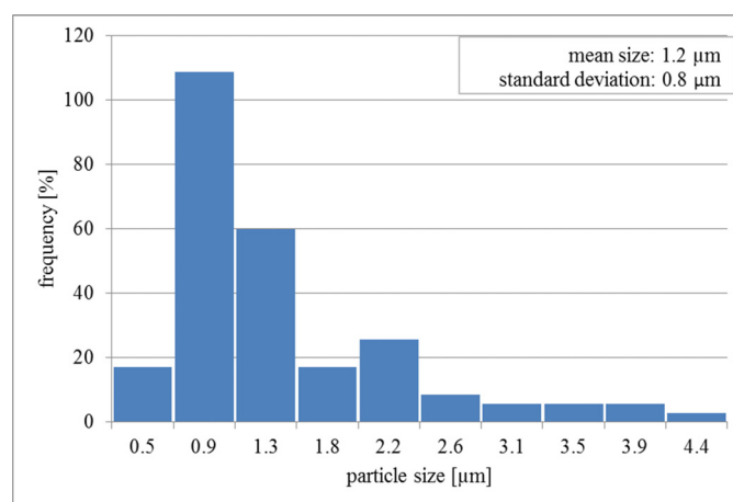
Fig. 6. Analysis of the ZrO_2 grain size in the zone I (frequency N [%] against diameter d_2 [ \mu\text{m} ])
