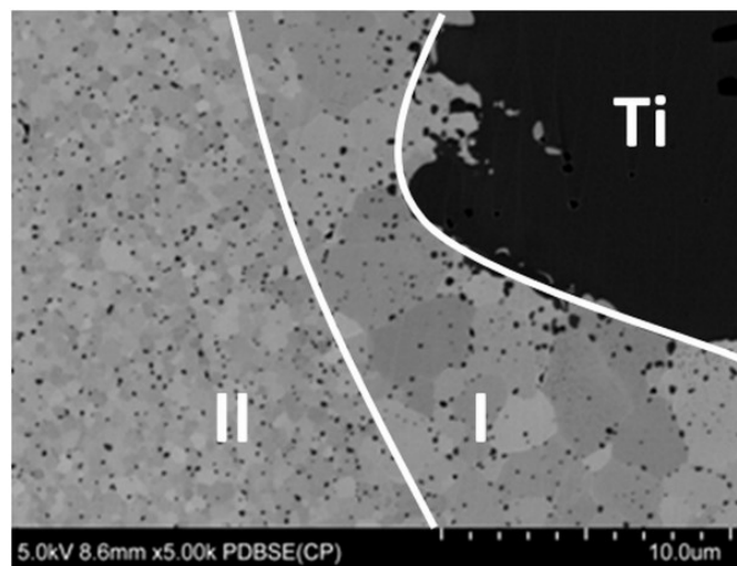
Fig. 5. Microstructure of the ZrO_2 – 10 vol.% Ti composite on the Ti/ ZrO_2 interface, SEM
