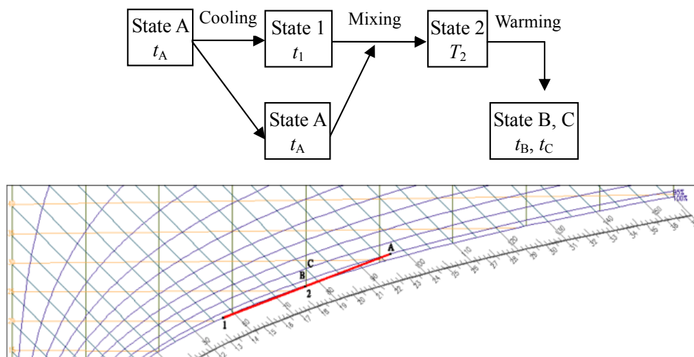
Fig. 9. Process of air handling at a time for air return system in air blending and cooling
