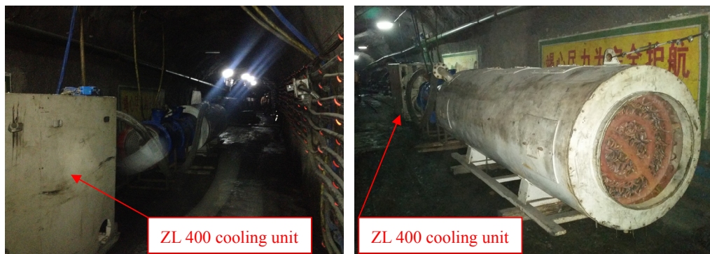
Fig. 11. ZL 400 cooling unit(direct action) used in underground mine
