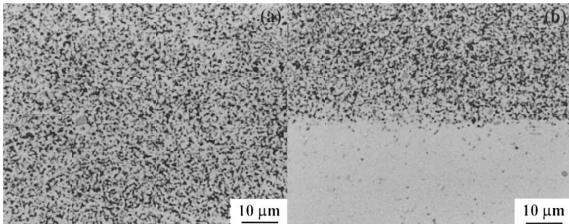
Fig. 2. OM image showing (a) uniform distribution of SiC particles (27 vol.%) in Al matrix, and (b) perfect bonding between composite layer and substrate (reprinted with permission from the publisher) [19]
