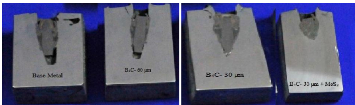
Fig. 19. Cross-sectional views of ballistic tested samples [111]
