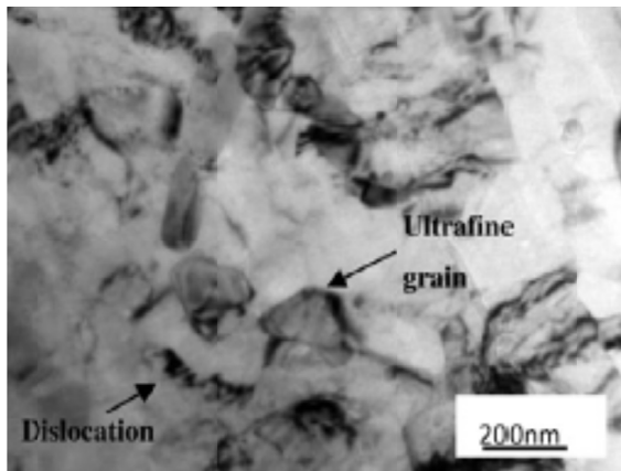
Fig. 1. TEM image showing the ultrafine grains and dislocations (reprinted with permission from the publisher) [69]
