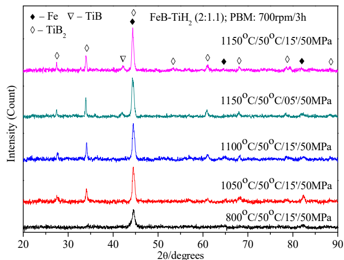
Fig. 3. XRD patterns of (FeB, TiB 2 ) powder compacts sintered by spark-plasma sintering at various sintering conditions (Sintering temperature/Heating rate/Sintering time/Sintering pressure)
