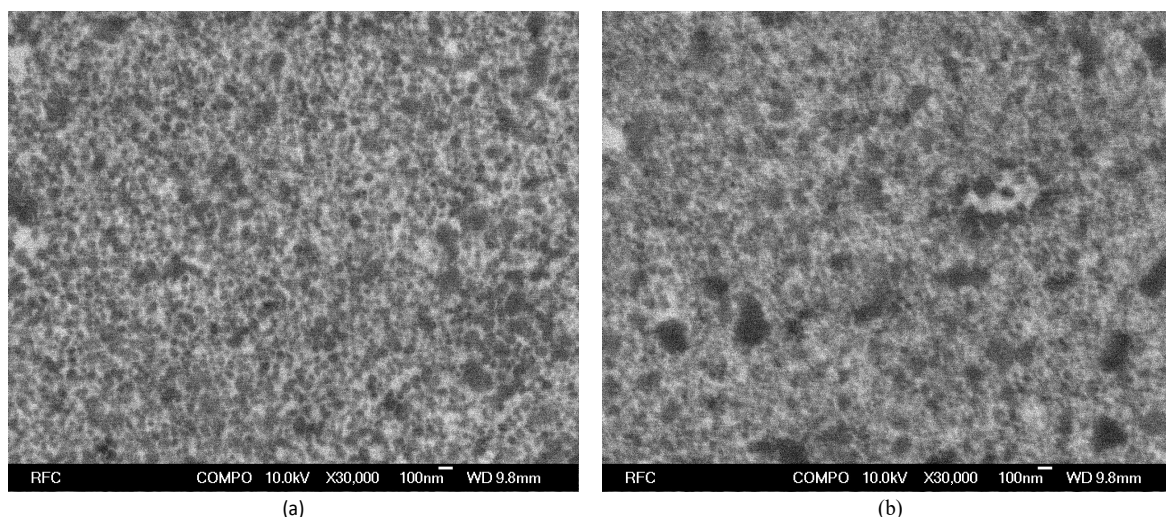
Fig. 4. FE-SEM backscattered-electron images of the polished cross-section of (FeB, TiB 2 ) powder compacts sintered at 1150°C for (a) 5 min. (98% RD) and (b) 15 min. (98% RD)
