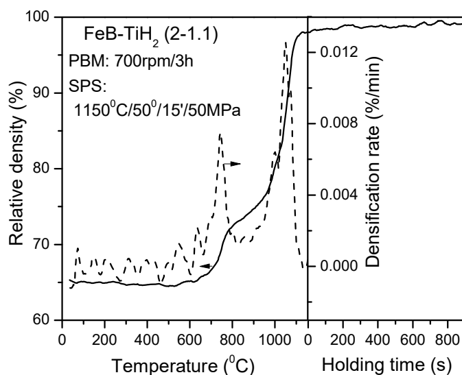
Fig. 1. Change of relative density (RD) and densification rate during the spark-plasma sintering process. The (\text{FeB}, \text{TiH}_2) powder compact was heated to 1150^\circ\text{C} at a heating rate of 50^\circ\text{C}/\text{min} under a sintering pressure of 50 MPa and then held for 15 min
