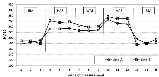
Fig. 7. Hardness HV10 of a weld joint BM - base material, HAZ - heat affected zone, WM - weld metal
