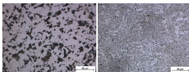
Fig. 8. The photo of the base material microstructure (left) and microstructure of HAZ (right)
