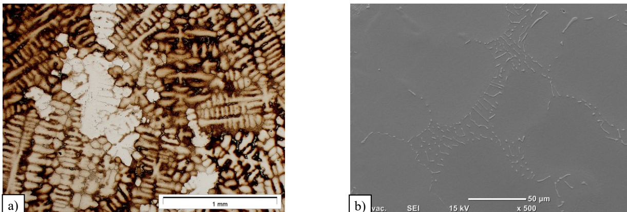
Fig. 2. Structure of the Inconel 713C castings used for the tests: a) casting macrostructure (LM), b) dendritic structure with visible carbides (SEM)
