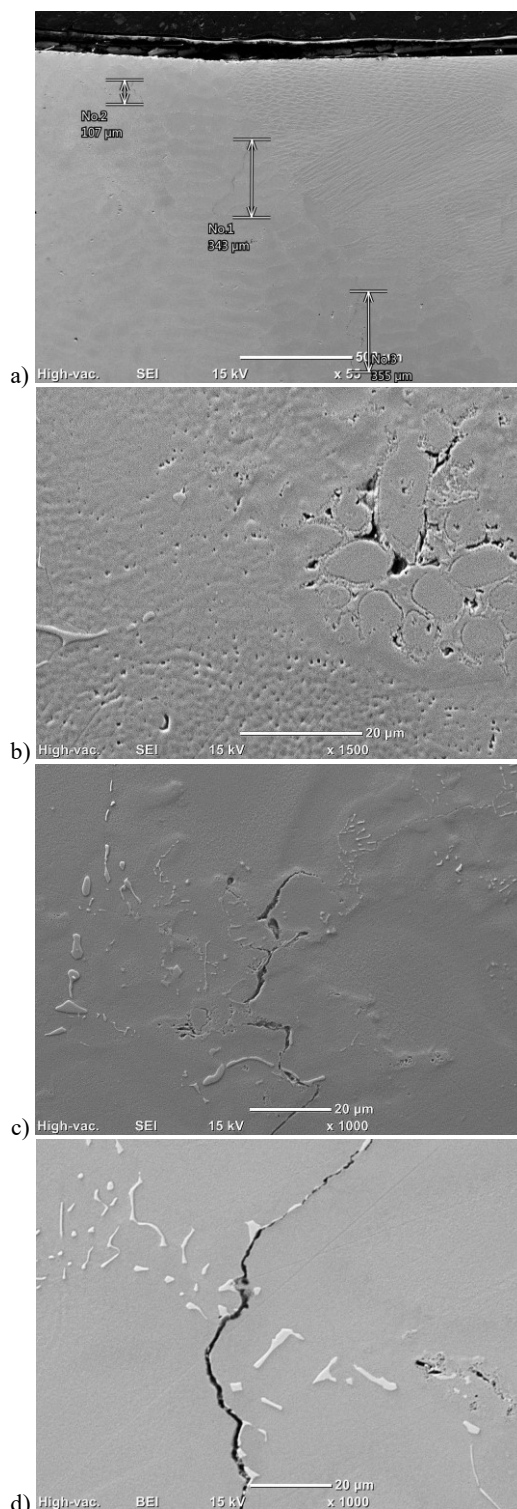
Fig. 7. Inconel 713C — cracks in the partially melted zone in the melting-affected zone: a) cracks identified in the PMZ, b) area of the partially melted eutectic mixture in the PMZ with visible discontinuities, c) interdendritic crack in the PMZ, d) crack along a phase \gamma dendrite boundary and along niobium carbides
