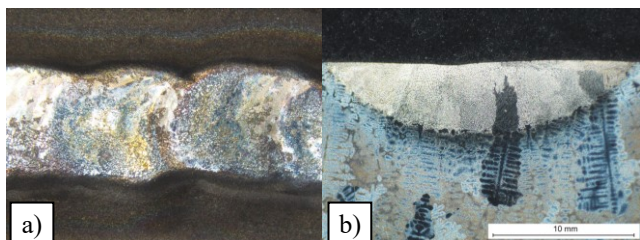
Fig. 5. Melting-affected zone surface (“face”) of an Inconel 713C precision casting (a), macrostructure of the melting-affected zone with a visible crack in the fusion zone (b)
