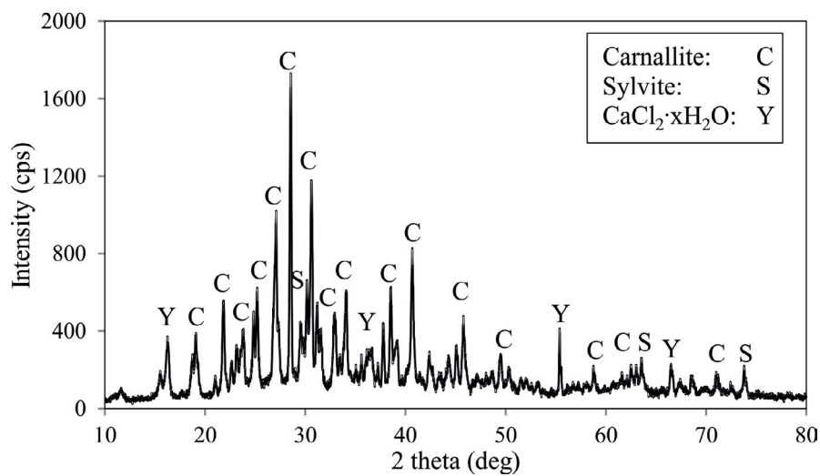
Fig. 12. XRD pattern of the synthesized carnallite
