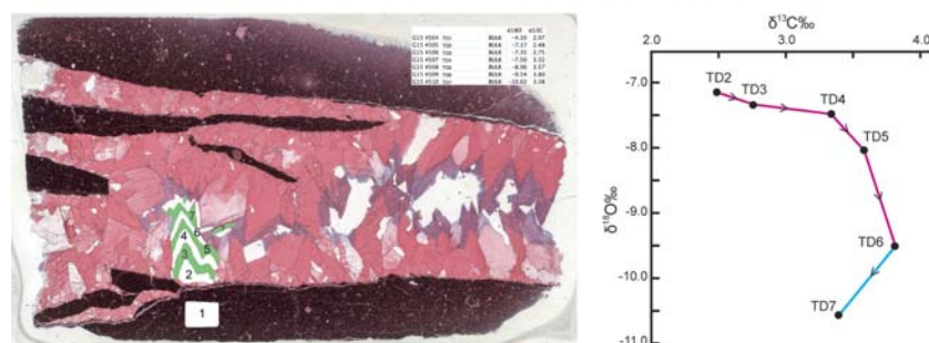
Text-fig. 20. A – Comparison of the average \delta^{18}\text{O} and \delta^{13}\text{C} values of the bulk calcite from the pressure dissolution marls and the adjacent chalk from the Upper Pink Band (Louth Member) at South Thoresby and Tetford with the sulfidized chalk at the same horizon in the Louth Member at Speeton. B. 1 – Stained thin section of a calcite vein from the Flamborough Head Chalk Formation at Selwicks Bay, Yorkshire, sampled for stable isotope analysis. This shows the non-ferroan nature of the main body of crystal growth but with a final phase of ferroan calcite. The growth stages and sampling zones in the calcite crystal analysed for stable isotope values are shown. 2 – Cross-plot of the \delta^{18}\text{O} and \delta^{13}\text{C} values shows that the calcite crystal initially grew with increasing \delta^{13}\text{C} values (suboxic pattern of Hu et al. 2012) and then in its final stages these values started to decrease in the ferruginous zone (anoxic pattern of Hu et al. 2012)
