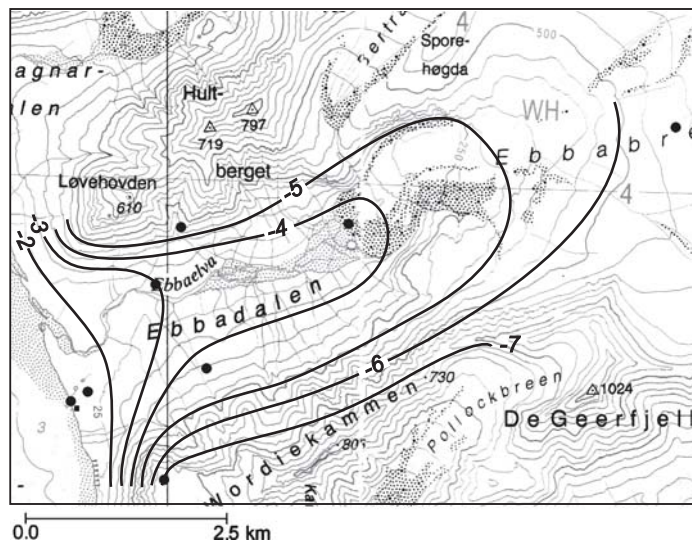
Fig. 14. The lowest wind-chill temperature (°C) observed in the Ebba Valley region during the studied period. Values of July 21 are averaged from 1 a.m. to 3 a.m.
