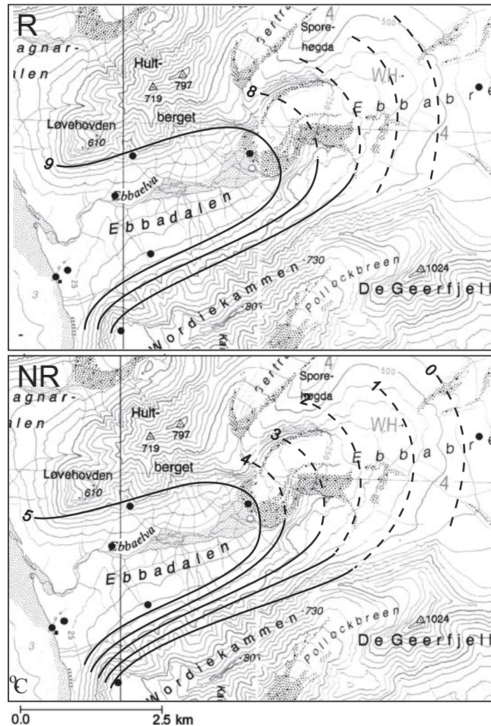
Fig. 5. Air temperature (°C) in the Ebba Valley region averaged for radiation days (R) and non-radiation days (NR).
