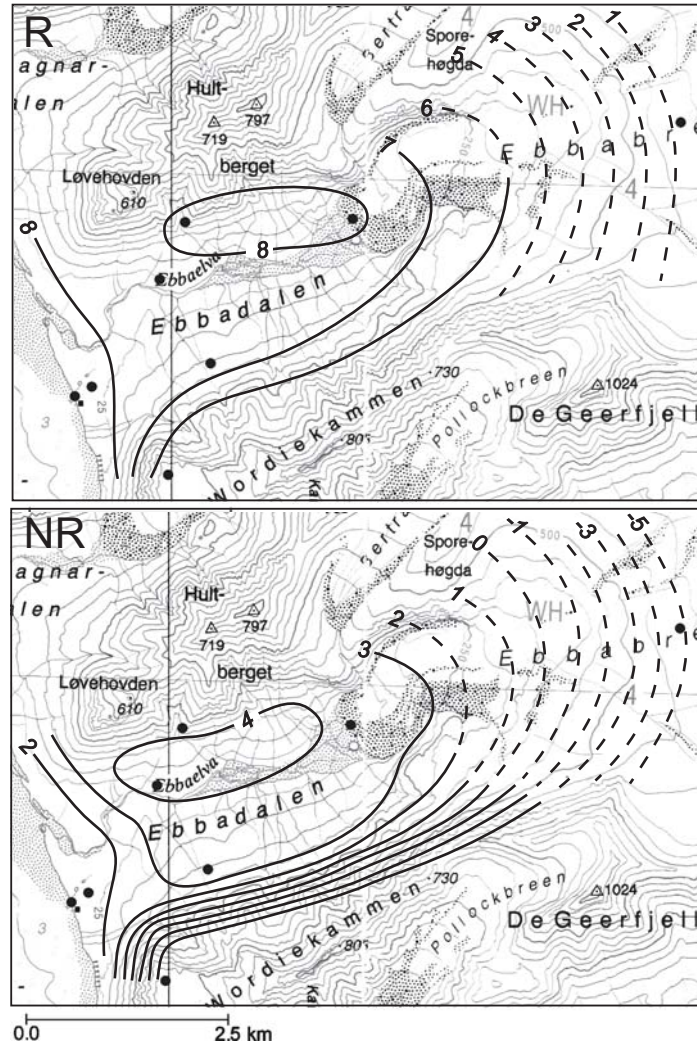
Fig. 12. Wind-chill temperature (°C) in the Ebba Valley region averaged for radiation days (R) and non-radiation days (NR).
