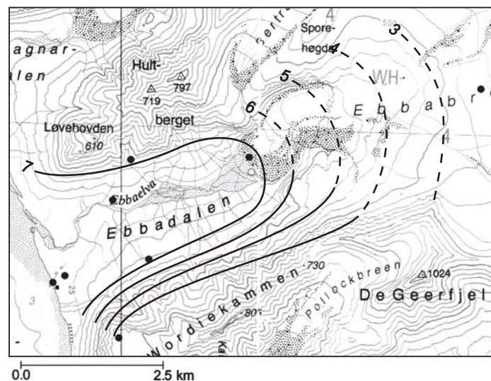
Fig. 2. Mean air temperature (°C) in the Ebba Valley region for all days of the studied period (July 10–25, 2009).
