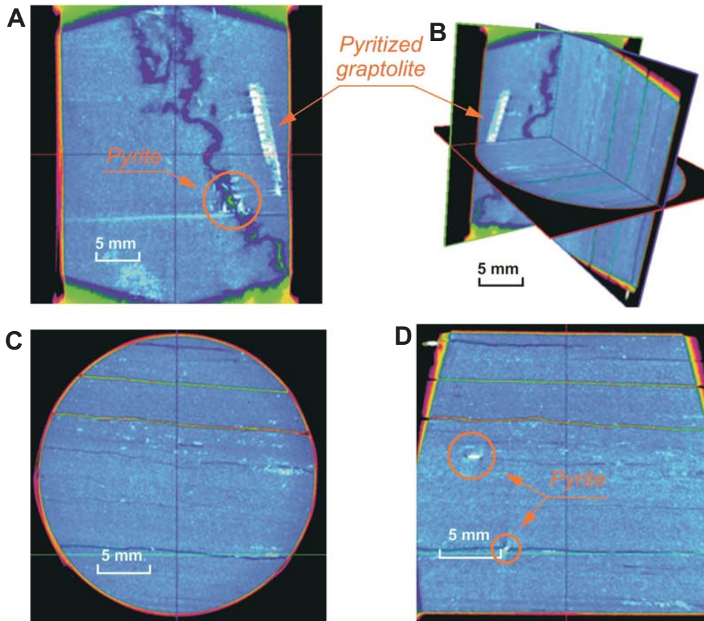
Text-fig. 6. Sections of sample 1, depth 2871.40 m, Opalino core, in the region where a graptolite fossil was detected, due to the contrast of linear attenuation coefficients. A – Longitudinal section parallel to the height of the sample. B – Overview of all sections. C – Cross-section perpendicular to the height of the sample. D – Longitudinal section parallel to the height of the sample and rotated 90 degrees to section A
