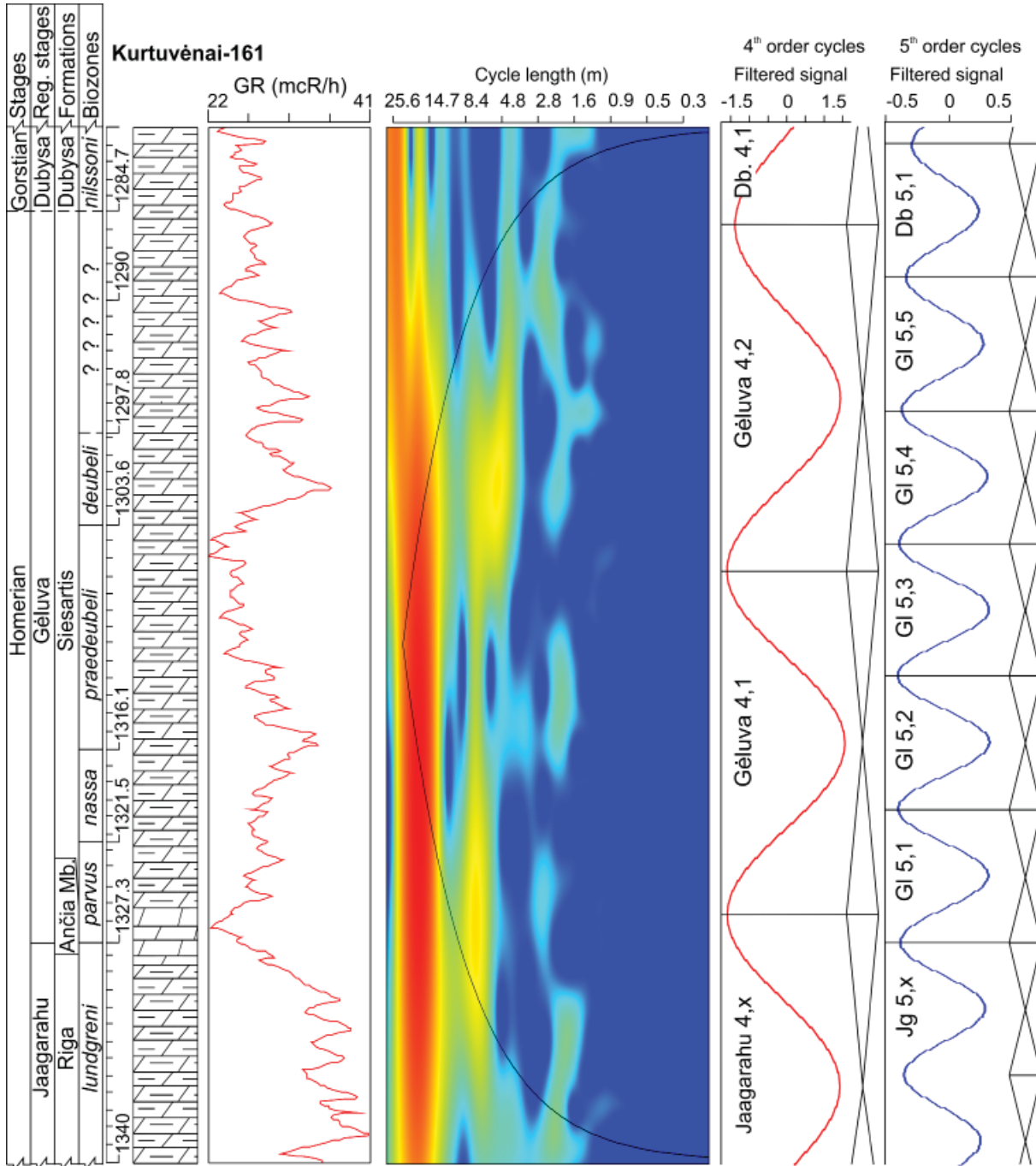
Text-fig. 6. Upper Homerian biostratigraphy, lithology, gamma-ray log data, wavelet scalogram and filtered cycles in the Kurtuvėnai-161 well. Legend see Text-fig. 3
