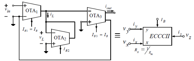
Fig.4. Building ECCCCII from OTA
