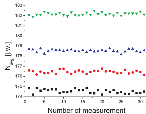
Fig. 13. Average brightness N_{avg} for selected settings of the sharpness for I_F = 20 mA at r = 100 mm for white diode LED5WW.
