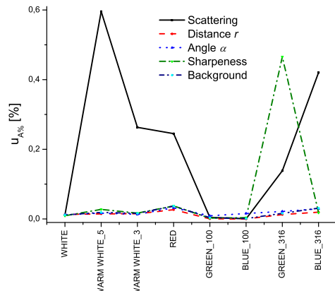
Fig. 17. Comparison of the values of the relative standard uncertainty u_{A\%} of results obtained from the registration with CCD camera for selected factors
