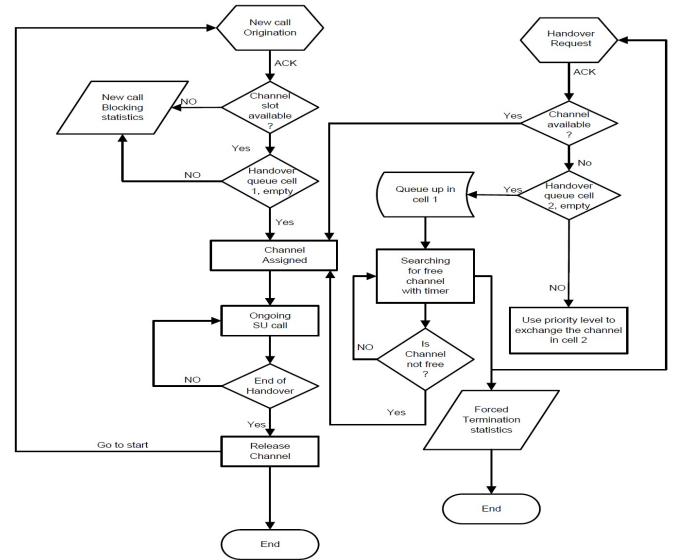
Fig. 3. Flow chart of the handover protocol/procedure.
