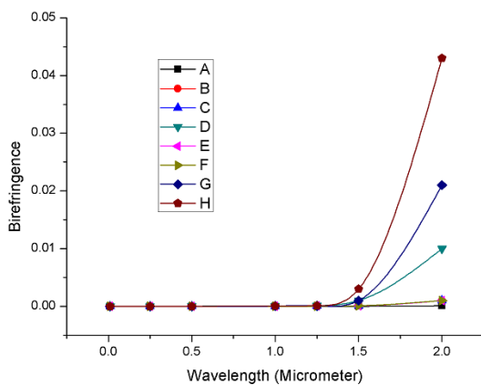
Fig. 3. Birefringence
