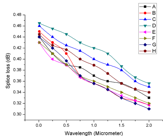
Fig. 5. Splice loss
