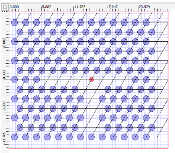
Fig. 1 (a). PCF structure A
