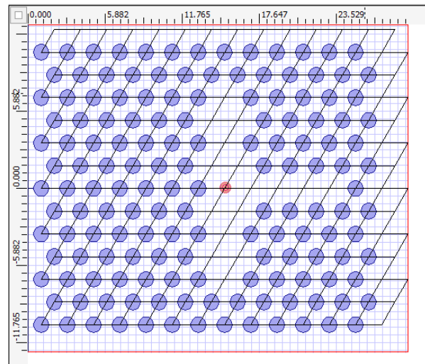
Fig. 1 (b). PCF structure B
