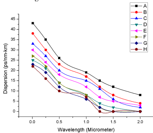
Fig. 2. Dispersion behavior
