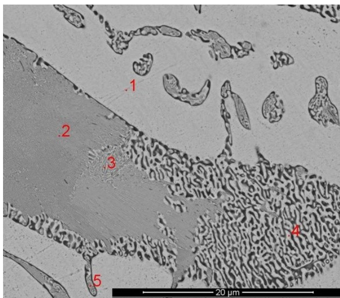
Fig. 5. Microstructure of Zn-Al-Cu cast alloy with Ce addition, cooling rate 0.1^{\circ}\text{C}/\text{s}
