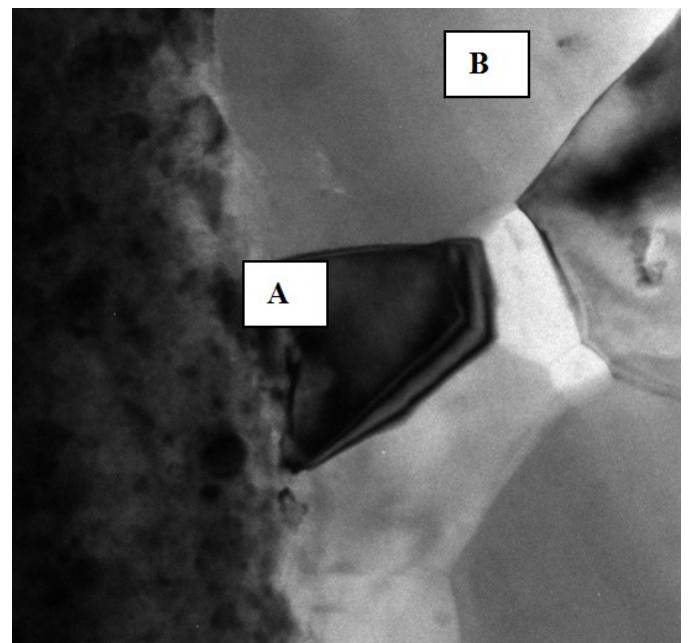
Fig. 6. Microstructure of Zn-Al-Cu alloys with Ce addition, grain boundary, bright field, TEM analysis
