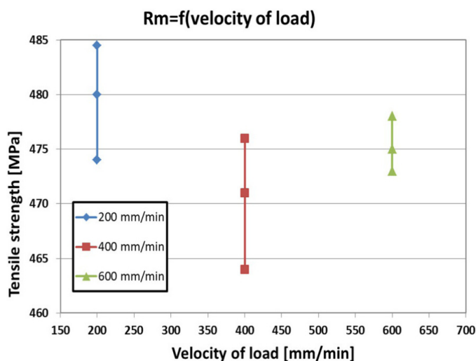
Fig. 2. Relationship between ultimate tensile stress and velocity of the load under tensile test
