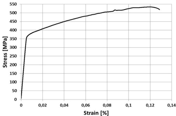
Fig. 1. Stress-strain curve for the RSA-501 aluminium alloy
