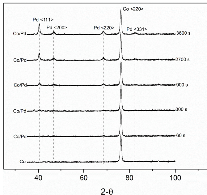
Fig. 5. XRD patterns of cobalt coatings after galvanic displacement surface modification for different time in palladium chloride solution
