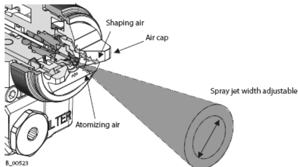
Fig. 3. The principle of hydrodynamic spraying [18]
