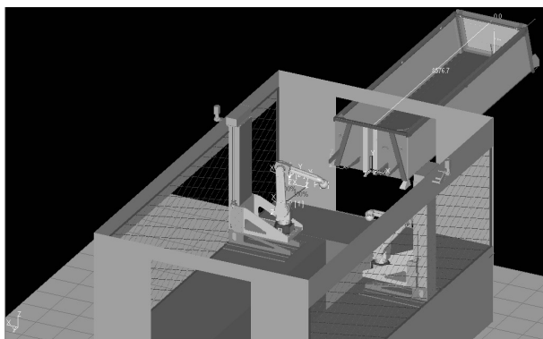
Fig. 7. View of load-carrying box situated in the painting chamber [5]
