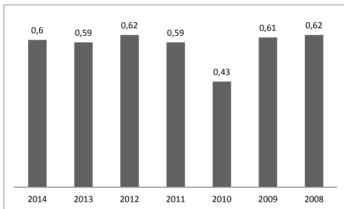
Fig. 2. Fuel consumption efficiency ratios for Glišno Gravel Pit [l/t].
