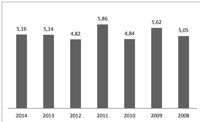
Fig. 3. Electricity consumption efficiency indicators for Glišno Gravel Pit [kwh/t].
