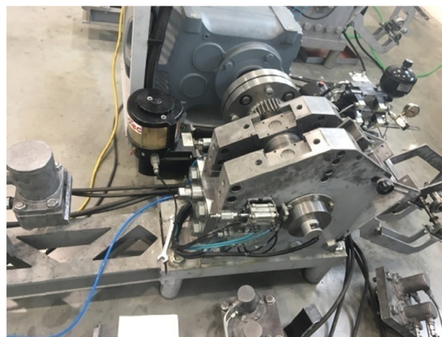
Fig. 1. a.) Principle of the DRECE process; 1 – feed roller, 2 – pressure roll, 3 – forming tool, 4 – forming tool with forming angle ( \alpha = 108^\circ ), 5 – sheet sample; b.) DRECE equipment
