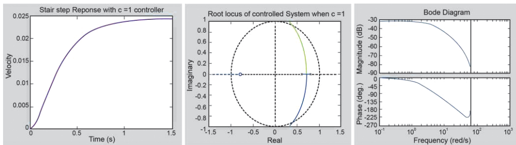
Fig. 1. Step response, root locus, and Bode plot of closed loop DC motor system angular velocity
