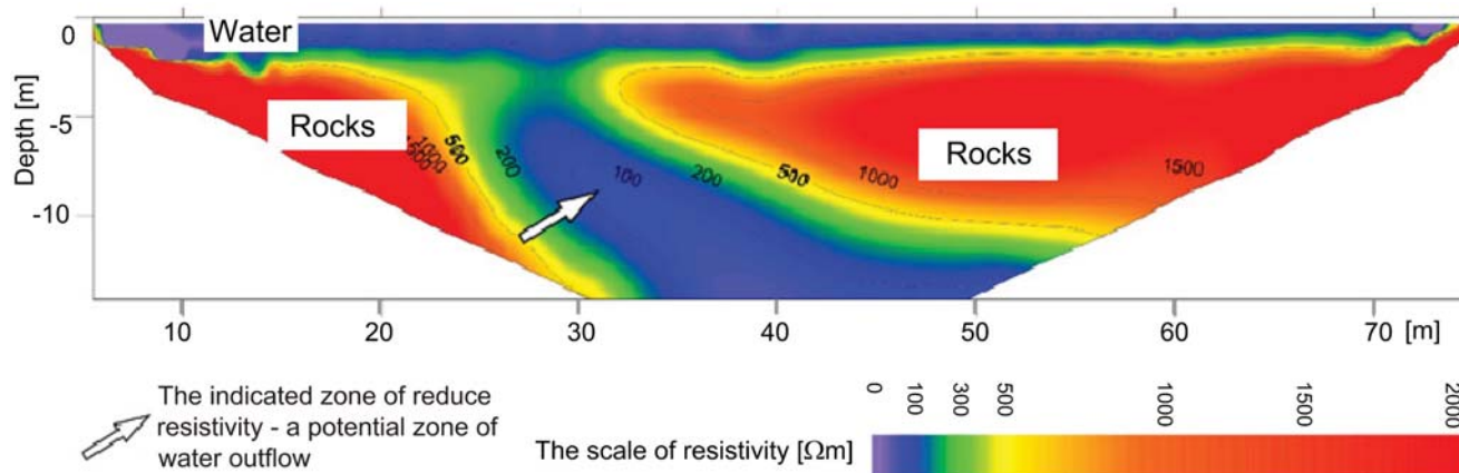
Fig. 8. ERT profile with anomalies in the lake bottom.
