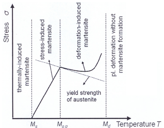
Fig. 1. Schematic diagram of the martensitic transformation induced by stress, strain and temperature [1,2]
