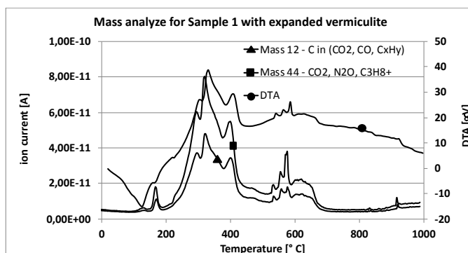
Fig. 7. Molar mass 12 and 44 measurement and DTA heat evolution from Sample 1
