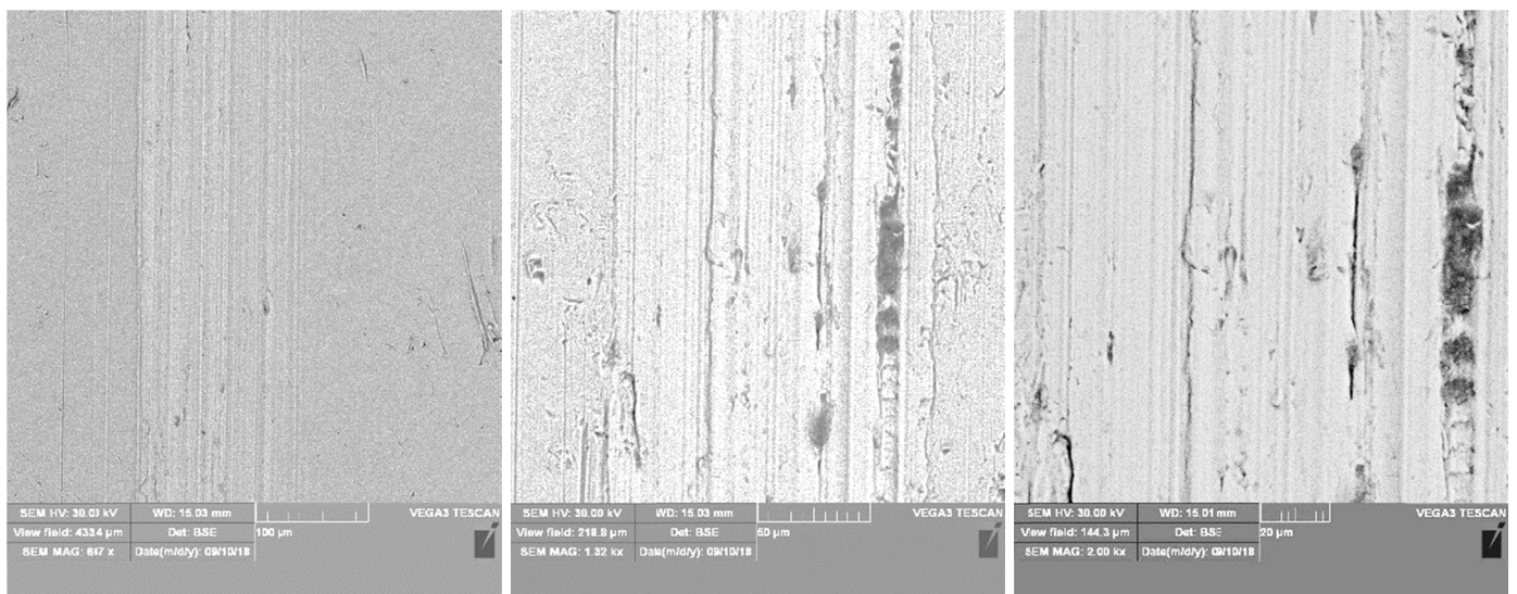
Fig. 15. Trace of wear for steel-steel material pair in the presence of scale
