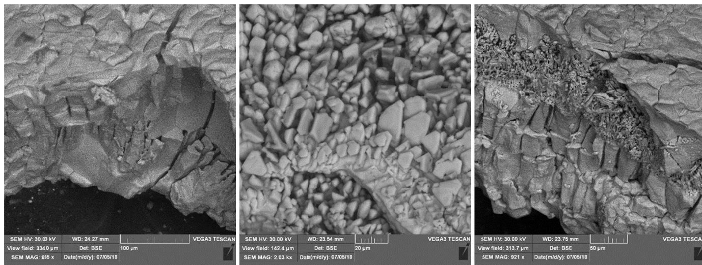
Fig. 10. Surface topography of scale chipped from forging material – steel C45
