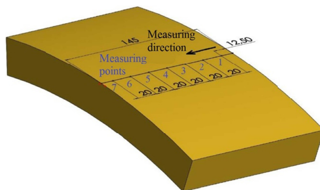
Fig. 2. Scheme of measuring direction and probe position for experiment
