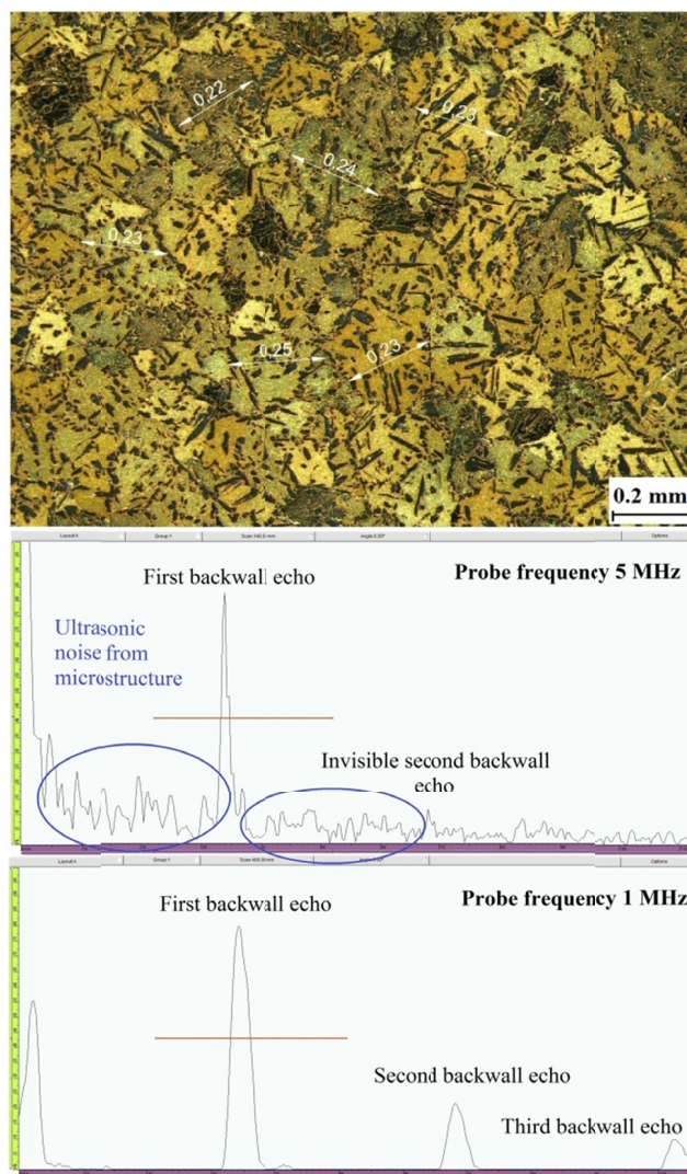
Fig. 5. Brass microstructure in point No. 2 (top), 5 MHz echogram (middle) and 1.00 MHz echogram (bottom)
